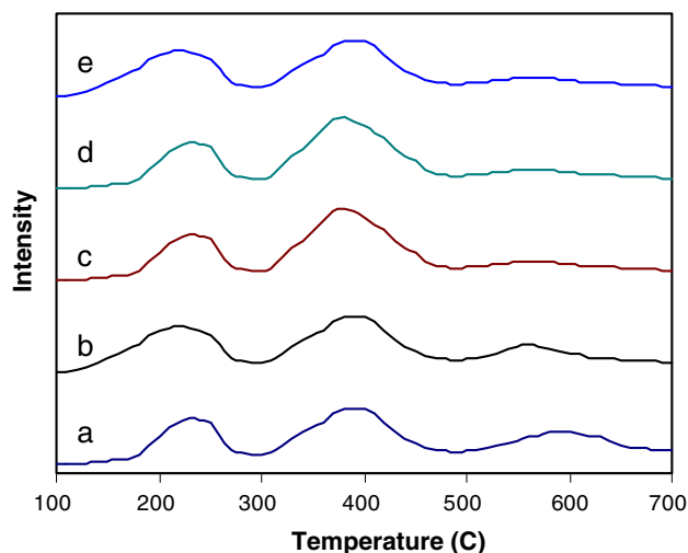
Fig. 3 \text{NH}_3 -TPD profile of H-Mordenite and of Al-modified H-Mordenite zeolites; (a) parent, (b) Al-modified HM (2 wt%), (c) Al-modified HM (5 wt%), (d) Al-modified HM (8 wt%) and (e) Al-modified HM (10 wt%)
